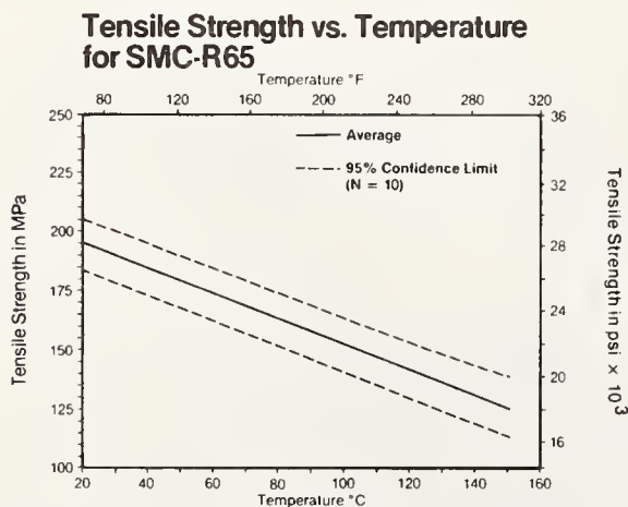
Fig. 7 - Tensile strength versus temperature for SMC-R65
